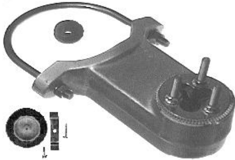
Signal Mount Assy w/grommet and sealing cap #7328 Nat finish,blk closure #7534 Nat finish,blk closure, SS hdwr #6367 Yellow,yel closure
